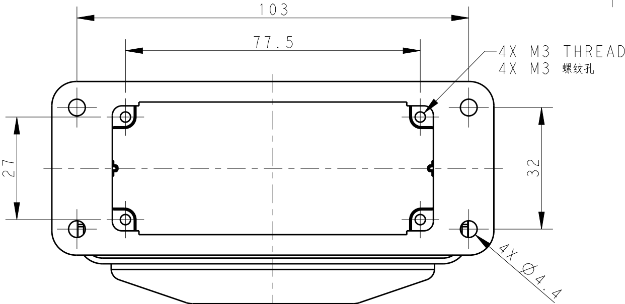
PANEL CUT OUT
