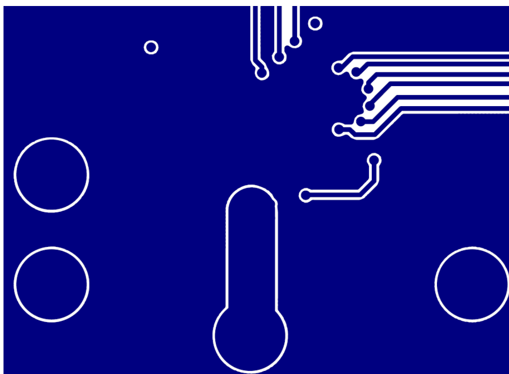
BOTTOM VIEW
