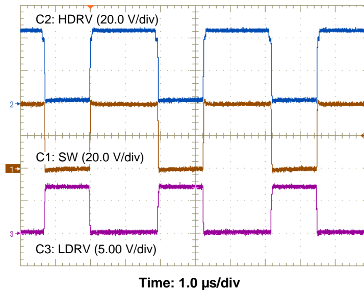
Figure 17. Gate-Drive Signals
