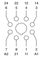
Terminal Arrangement
