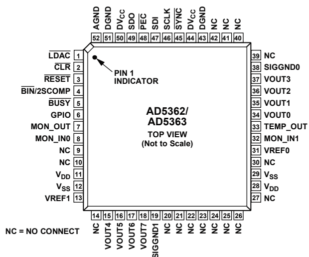
Figure 7. 52-Lead LOFP Pin Configuration
