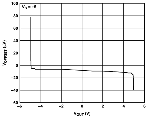
Figure 20. Input Error Voltage vs. Output Voltage
