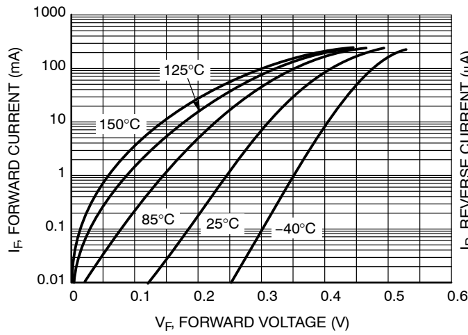
Figure 2. Forward Voltage
