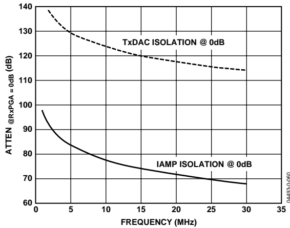
Figure 23. Rx to Tx Full-Duplex Isolation @ 0 RxPGA Setting (Note: ATTEN @ RxPGA = x\text{ dB} = ATTN @ RxPGA = 0\text{ dB} - RxPGA\text{ Gain} )
