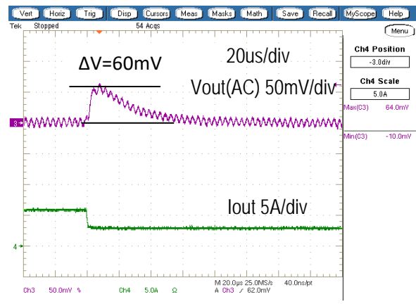
Step Load Transient Response (Vin=12V, Vout=3.3V, Cloud=400uF, Iout=6A to 3A, 2.5A/us)
