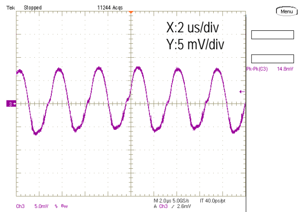
Output Ripple and Noise (Vin=12V, Vout=3.3V, Iout=6A, Cloud=400uF, ScopeBW=20MHz)
