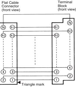
Connection Diagram
