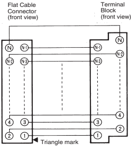
Connection Diagram
