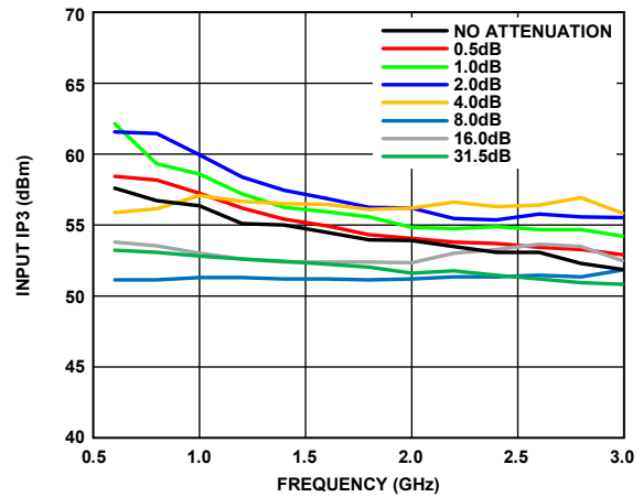
Figure 23. Input IP3 vs. Frequency, Major States Only
