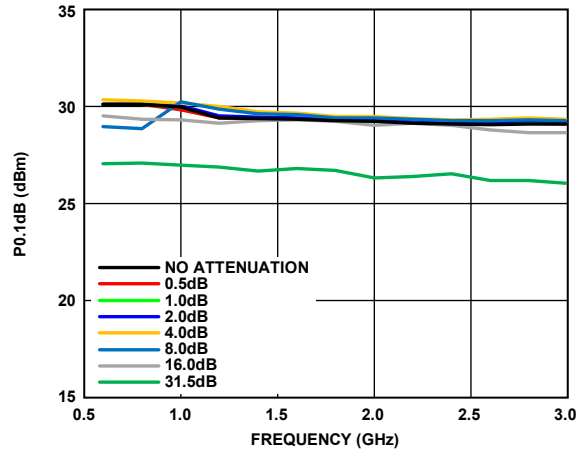
Figure 21. P0.1dB vs. Frequency, Major States Only
