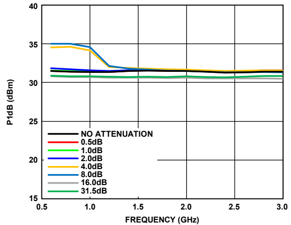
Figure 22. P1dB vs. Frequency, Major States Only
