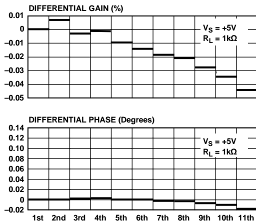
Figure 37. Differential Gain and Differential Phase, R_L = 1\text{k}\Omega
