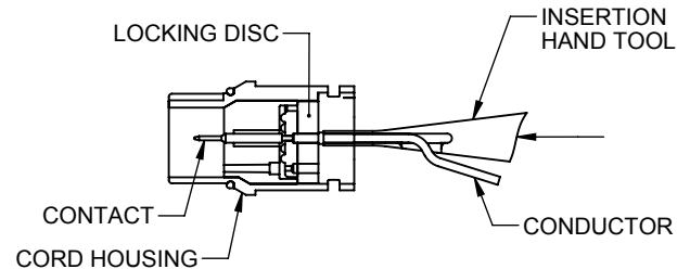
CORD WIRING SIDE VIEW
