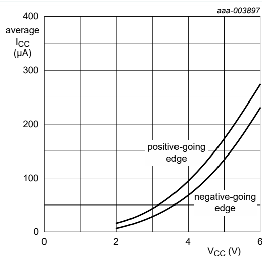
Fig. 12. Average additional supply current as a function of V_{\text{CC}} for 74HC132-Q100; linear change of V_i between 0.1V_{\text{CC}} to 0.9V_{\text{CC}} .
