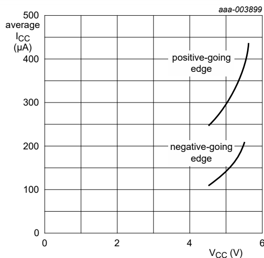
Fig. 13. Average additional supply current as a function of V_{\text{CC}} for 74HCT132-Q100; linear change of V_i between 0.1V_{\text{CC}} to 0.9V_{\text{CC}} .
