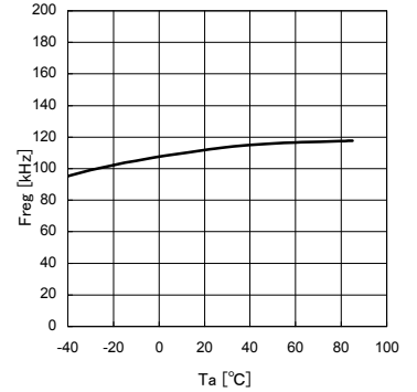
Fig.18 Switching
