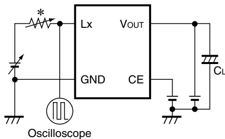
Test Circuit 3
