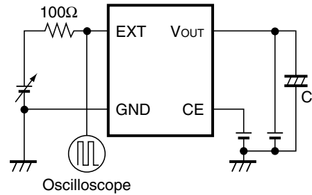
Test Circuit 4
