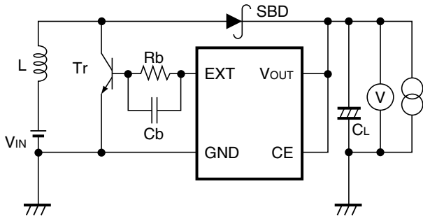
Test Circuit 1
