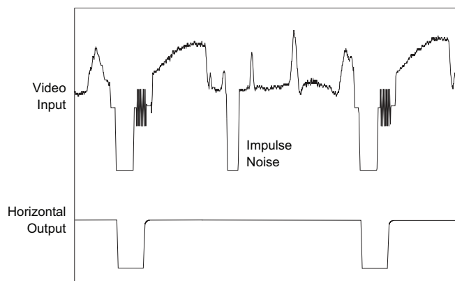
Figure 4-4: Horizontal Output
