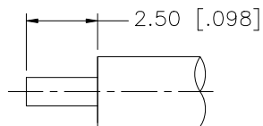
RECOMMENDED CABLE STRIPPING DIMENSIONS
