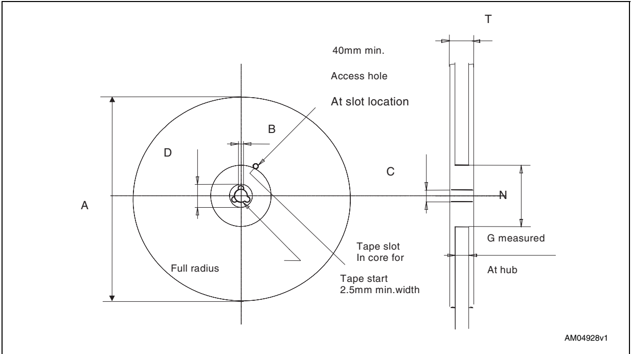
Figure 21. Reel schematic
