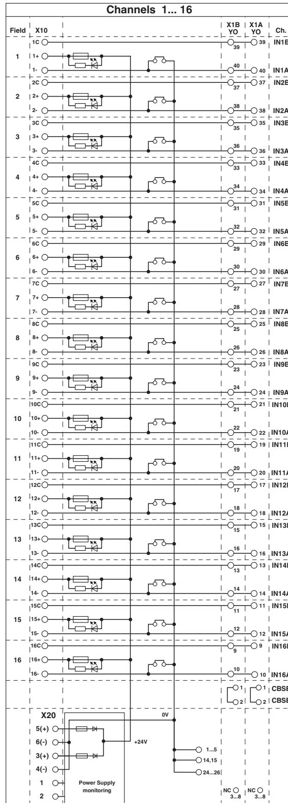
Circuit diagram
