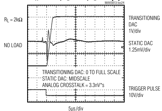
CHANNEL-TO-CHANNEL FEEDTHROUGH ( V_{DD} = 5V , V_{REF} = 4.096V (INTERNAL), T_A = +25^\circ\text{C} , R_L = 2k\Omega , C_L = 200pF )
