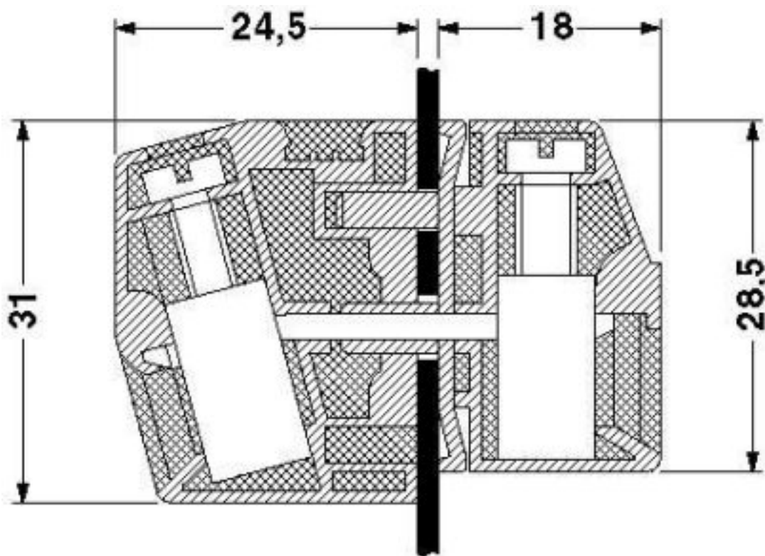
Dimensioned drawing
