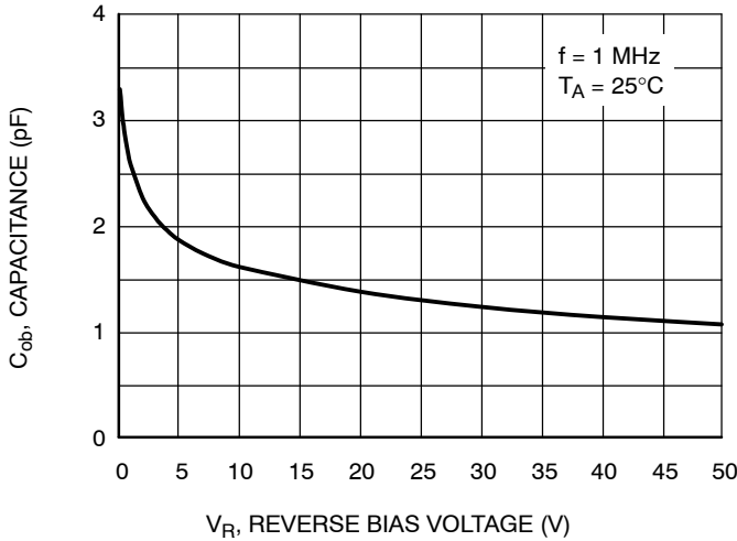
Figure 35. Output Capacitance
