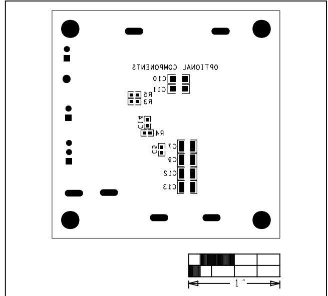
Figure 2. MAXM17505 EV Kit Component Placement Guide—Solder Side
