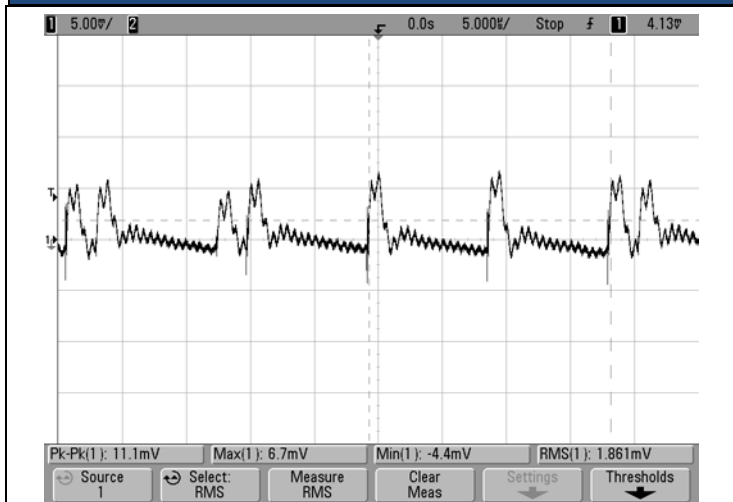
Ripple and Noise @25°C (Vin = 110V, Vout = nom., Iout = 0, Cloud = 0, ScopeBW = 20MHz)
