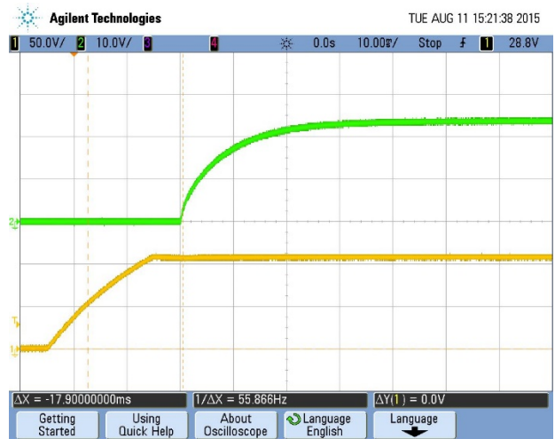
Turn-on transient at full load current (10 mS/div, Top Trace: Vout, 10V/div; Bottom Trace: Vin, 50V/div)
