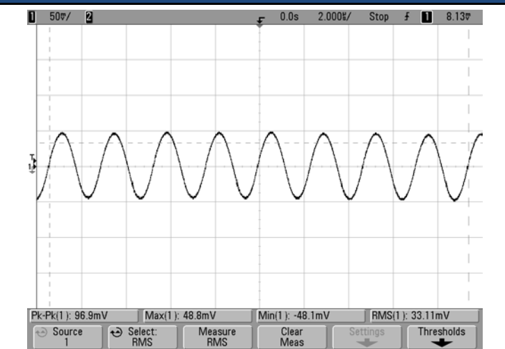
Ripple and Noise @25°C (Vin = 110V, Vout = nom., Iout = 20A, Cload = 0, ScopeBW = 20MHz)
