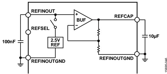
Figure 46. Reference Circuitry
