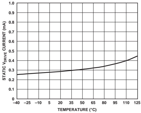
Figure 38. Static V_{DRIVE} Current vs. Temperature
