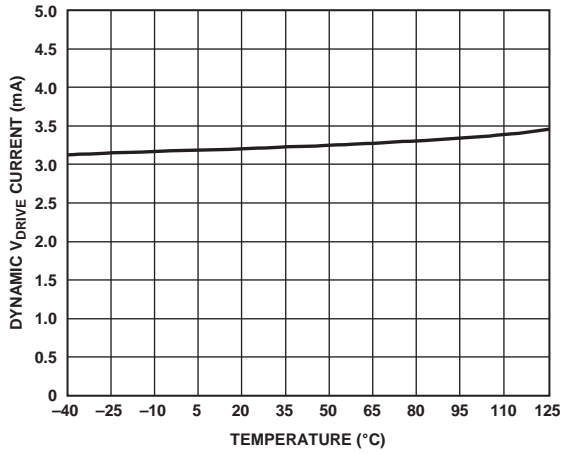
Figure 37. Dynamic V_{DRIVE} Current vs. Temperature
