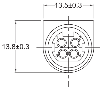
4 PIN CONFIGURATION
