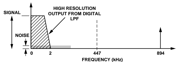
Figure 40. Noise Reduction due to Oversampling and Noise Shaping in the Analog Modulator
