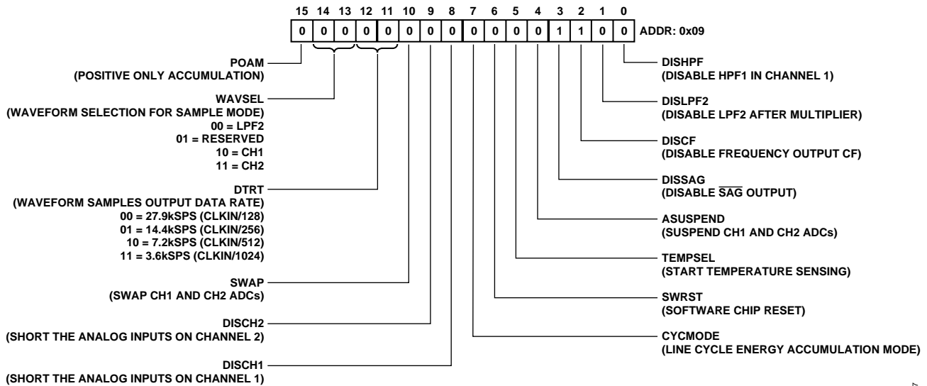
Figure 86. Mode Register
