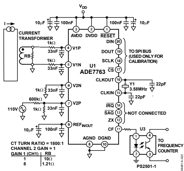
Figure 22. Test Circuit for Performance Curves with Integrator Off
