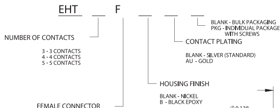
4 PIN
