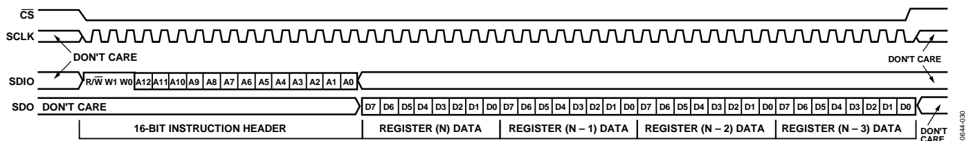
Figure 46. Serial Control Port Read—MSB First, 16-Bit Instruction, Four Bytes of Data
