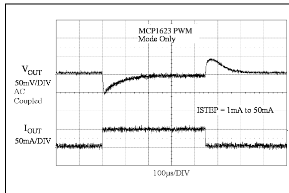
FIGURE 2-23: MCP1623 2.0V V_{OUT} Load Transient Waveforms.
