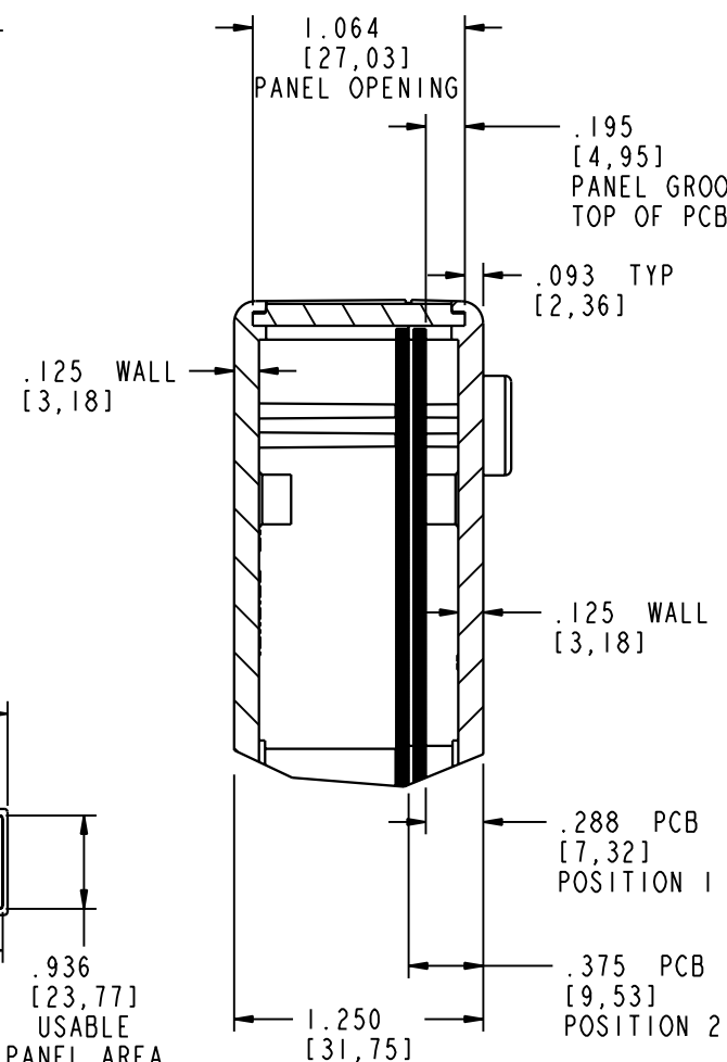
SECTION C-C
