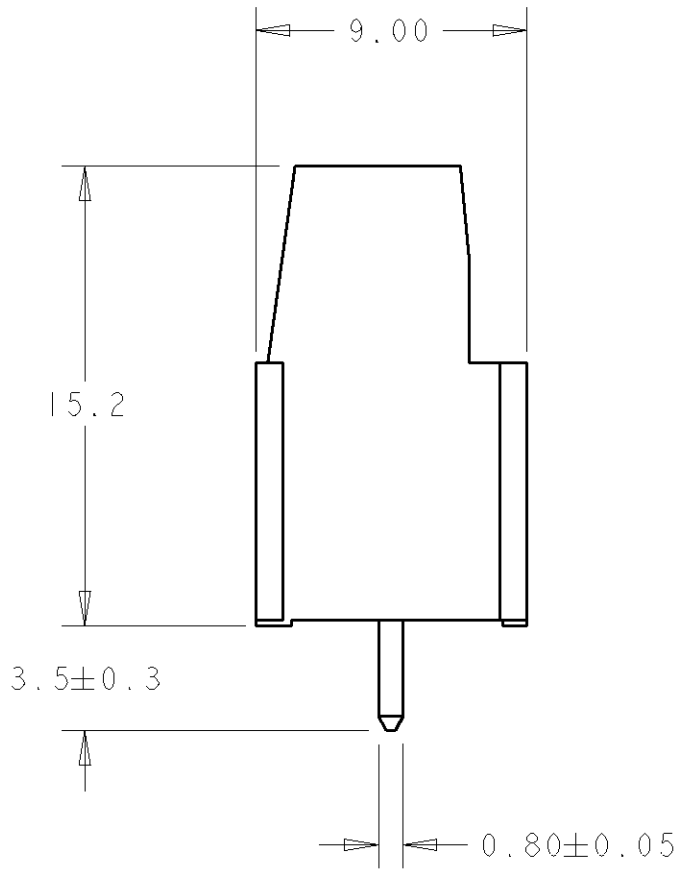
P/N 1546062-3 AS SHOWN
