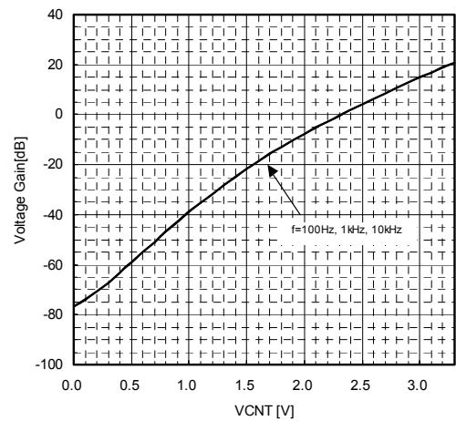
Voltage Gain vs. Control Voltage (Frequency) V_+=9\text{V} , V_{in}=-20\text{dBV} , R_L=100\Omega , T_a=25^\circ\text{C}
