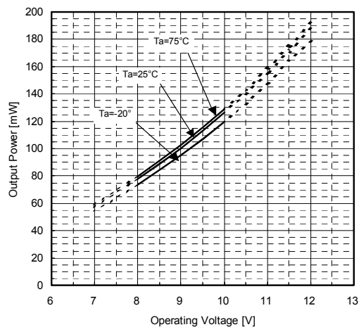
Output Power vs. Operating Voltage f=1\text{kHz} , THD=10\% , G_v=10\text{dB} , R_L=100\Omega , BW=400\text{Hz-30kHz}
