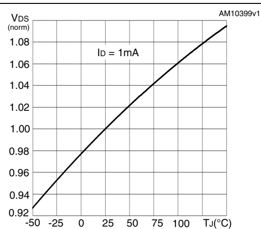
Figure 15. Normalized V_{DS} vs. temperature
