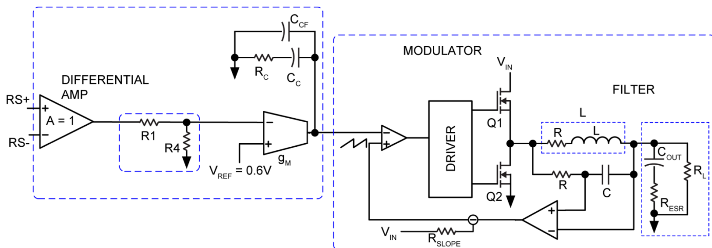
Figure 15. Valley Current Mode Loop Compensation
