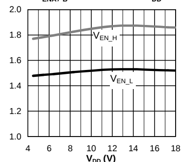
V_{\text{ENA}, \text{B}} Threshold vs. V_{\text{DD}}
