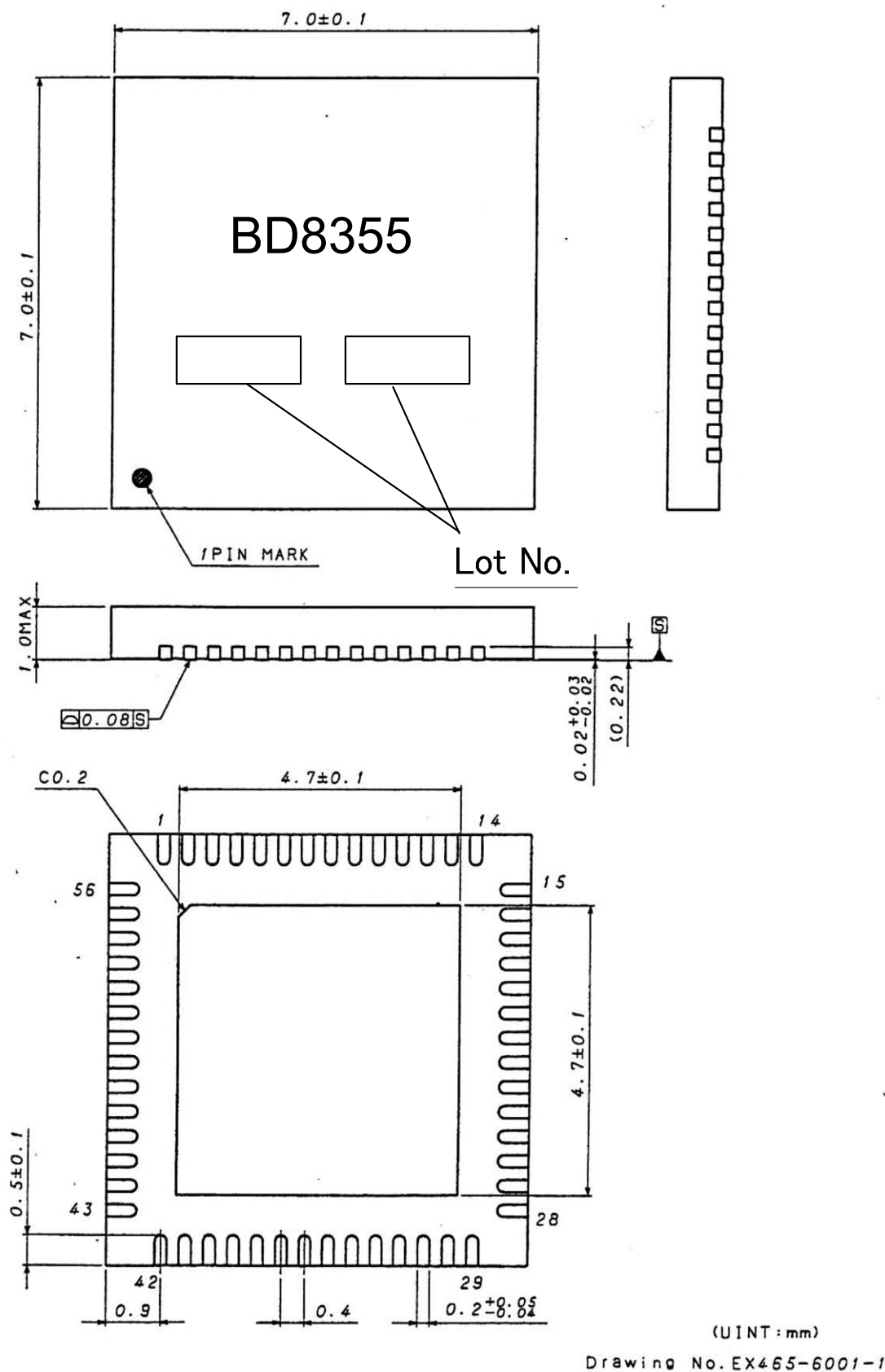
Fig. 1 Package dimension
