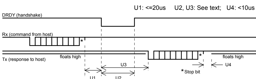
Figure 3-4 UART Timing
