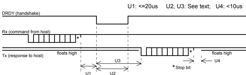
Figure 3-4 UART Timing
