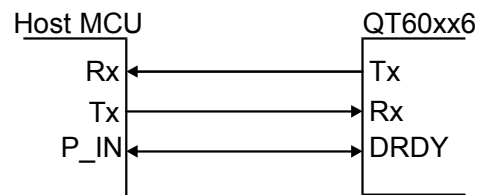
Figure 3-5 UART Connections
