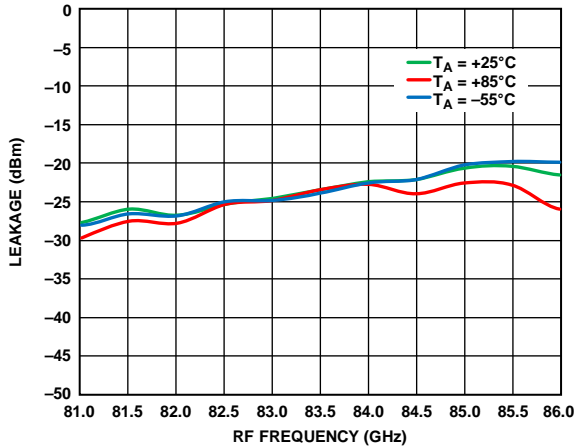
Figure 31. 6x LO Leakage at RFOUT vs. RF Frequency at Various Temperatures, I_{FIN} = 5 \text{ dBm} , LO = 2 \text{ dBm} , IF = 1000 \text{ MHz} , USB
