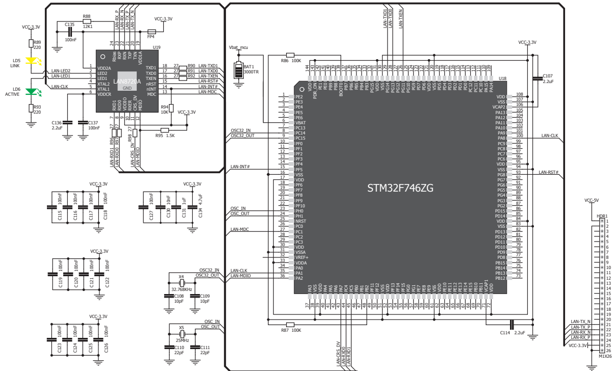
Figure 14-2: Ethernet transceiver module schematic
