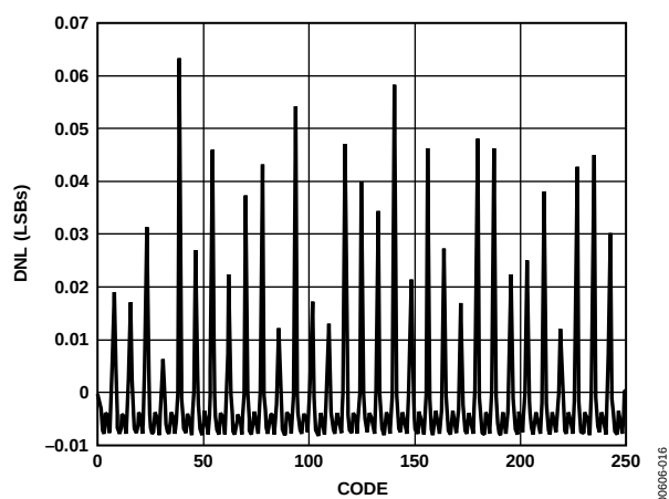
Figure 15. Typical DNL
