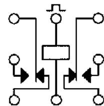
TERMINAL VIEW
