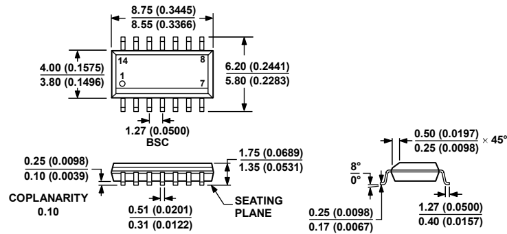
Figure 38. 14-Lead Standard Small Outline Package [SOIC_N] Narrow Body (R-14) Dimensions shown in millimeters and (inches)
